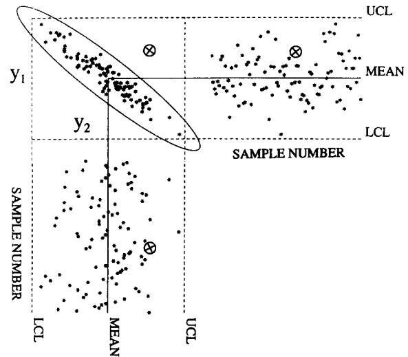
Figure 1. Quality control of two variables illustrating the misleading nature of univariate charts.
