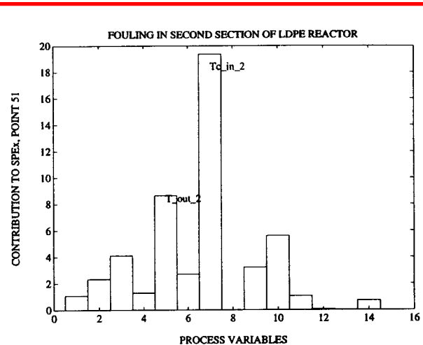
Figure 5. Contribution plot showing the process variable contributions to the SPE_x for point 51.
