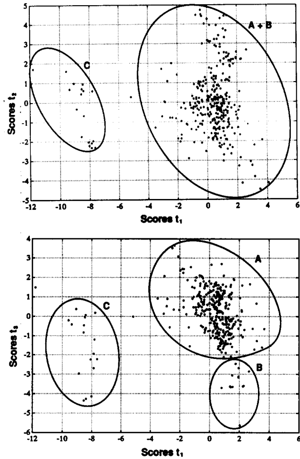
Figure 2. PLS scores plots for several hundred hours of operation of the rougher scavenger unit of a mineral flotation process. t_1 vs t_2 , and t_1 vs t_3 . (Hodouin et al. (1993); With permission from CIM Bulletin).
